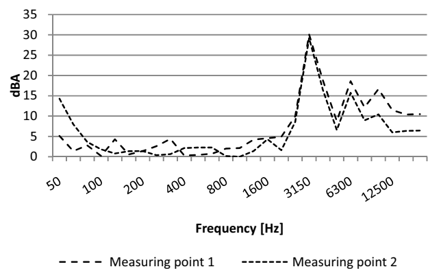
Fig. 3 Noise reduction by using CL-E1topsystem
